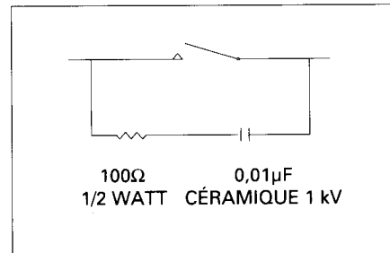
Figure 2.1 Circuit anti-étincelles
