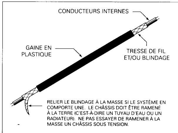
Figure 1.5 Fil audio blindé
